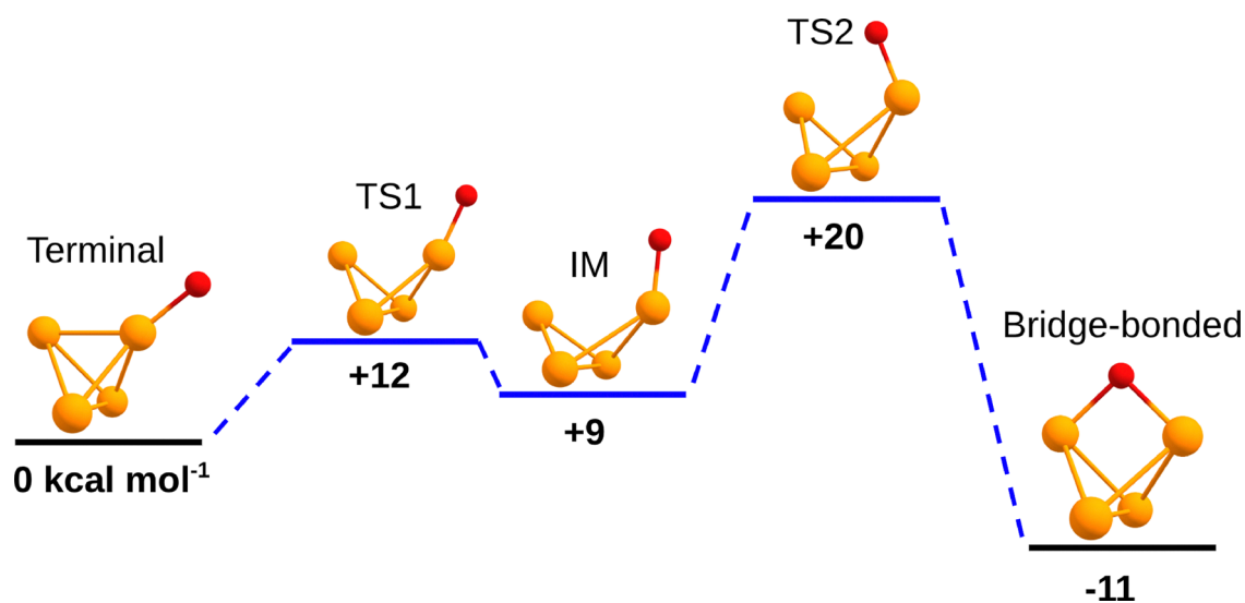
Fig. 2 CCSD(T)/cc-pV(T+d)Z//CCSD/cc-pV(T+d)Z stationary points along the T- \text{P}_4\text{O} \rightarrow B- \text{P}_4\text{O} reaction coordinate. TS denotes transition state and IM denotes intermediate.
